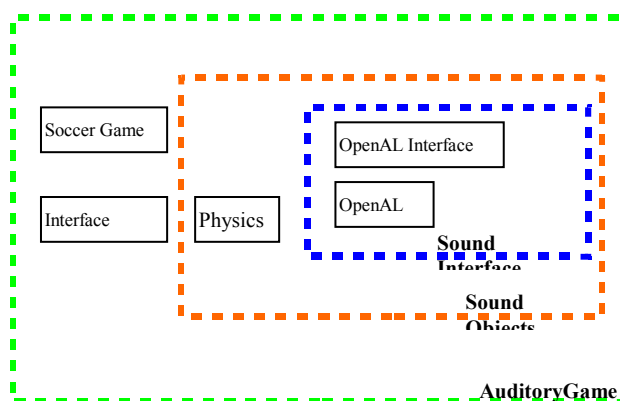
Figure 1. The architecture of the system consists of 3 layers: the Sound Interface, Sound Objects, and the Auditory Game
